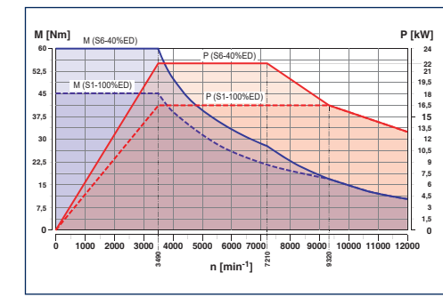
Milling spindle with max. 12000 rpm
