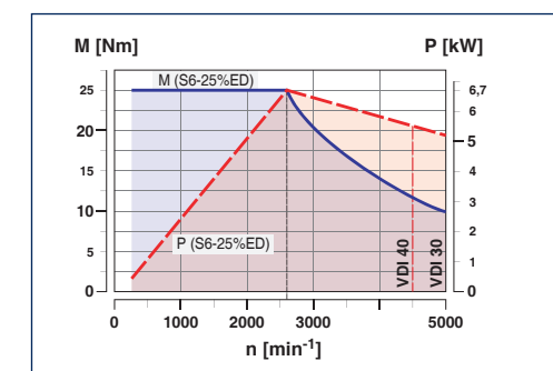
Milling drives in tool turret with VDI 30/40
